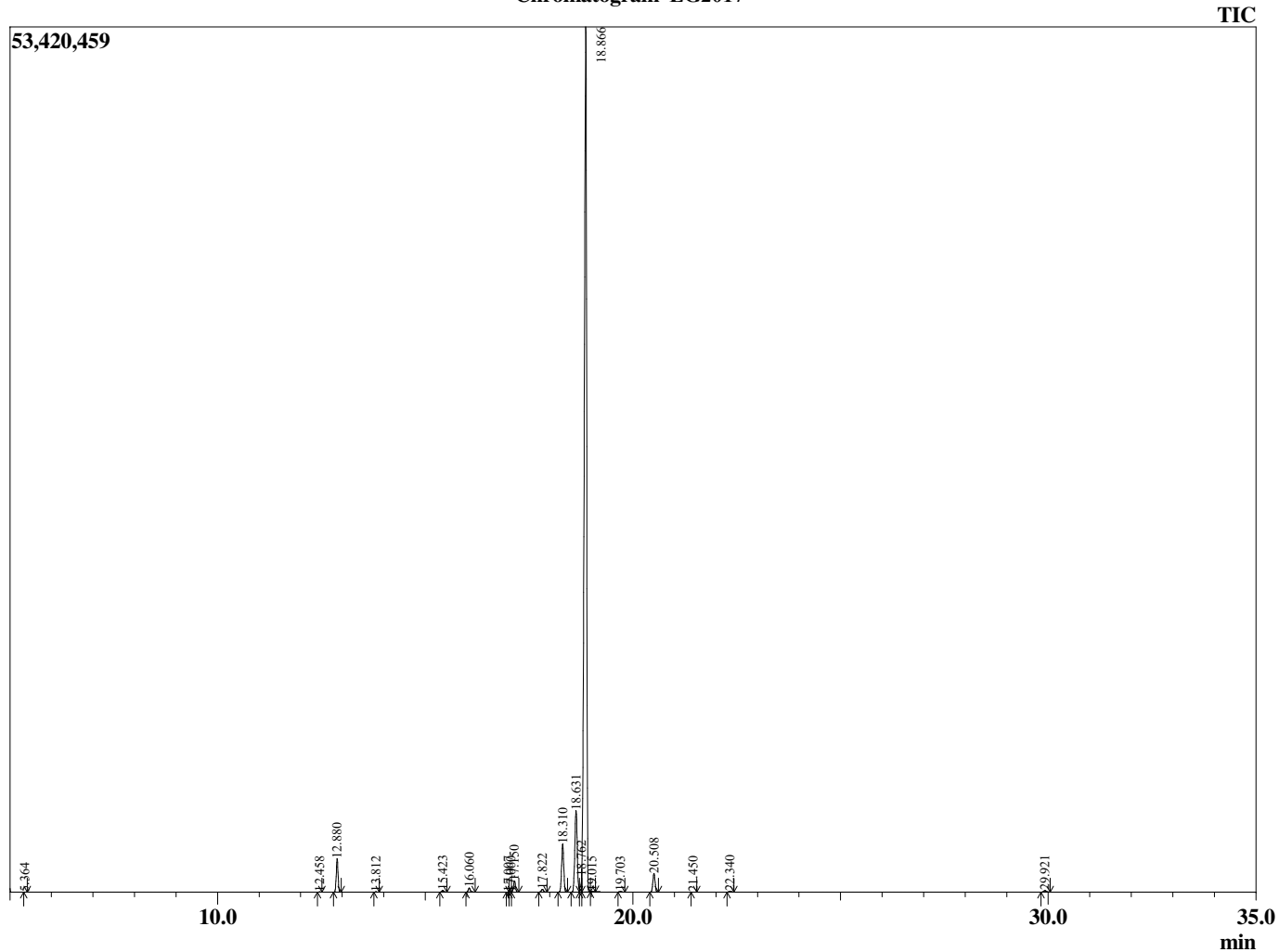
Chromatogram EG2017
